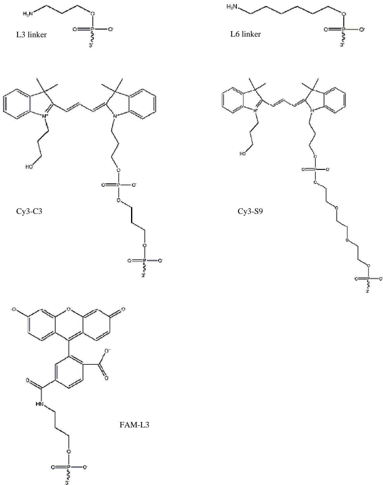
Figure S3. Chemical structures of various linker-dye combinations that were investigated.
